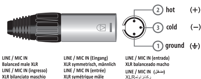
FLASH15A CONNEXIONS (FIG.2)
